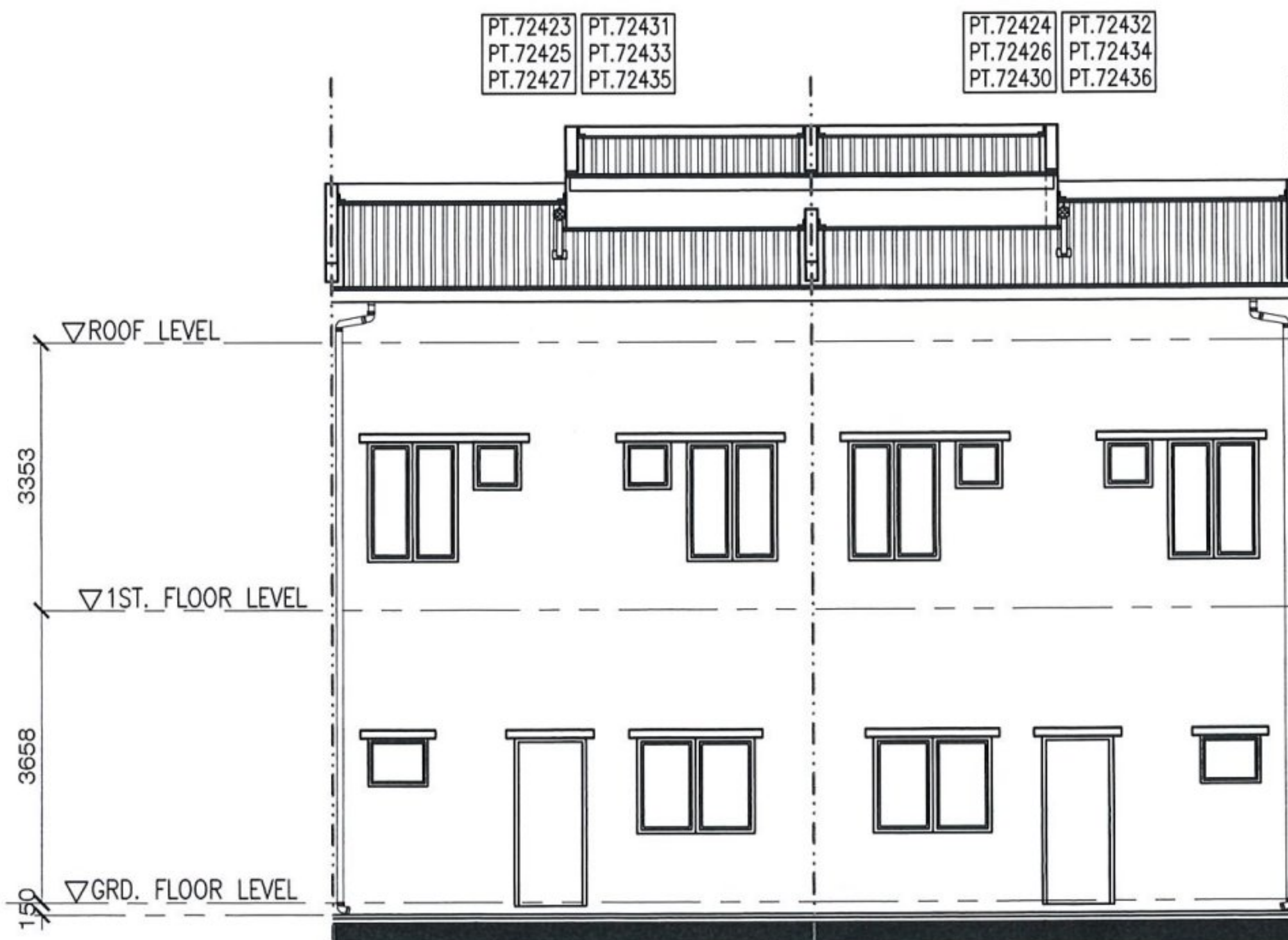
REAR ELEVATION
