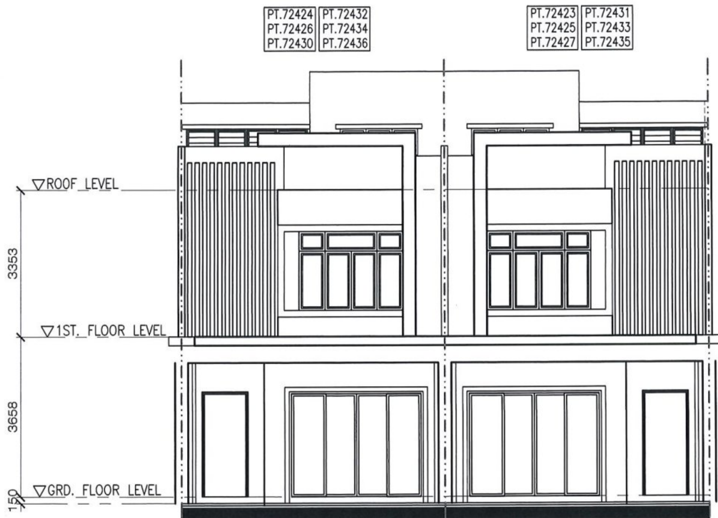
FRONT ELEVATION
