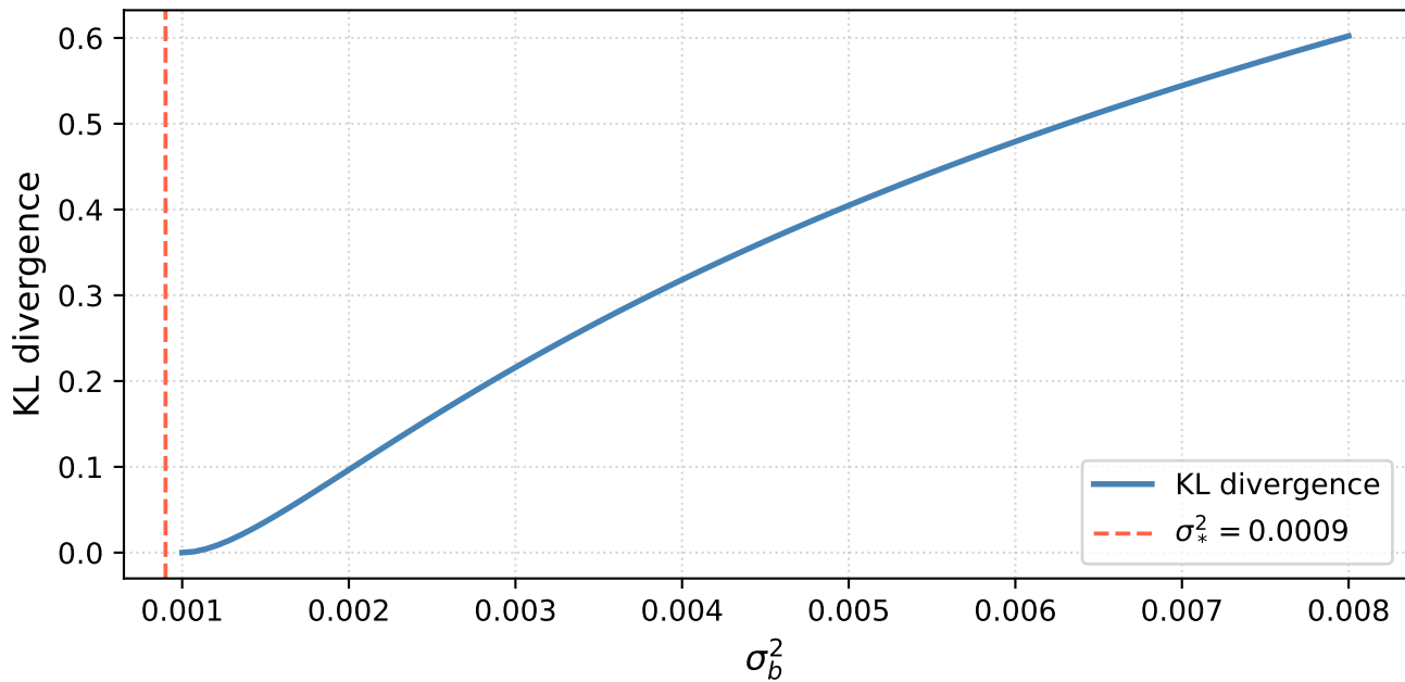
KL Divergence vs Variance (Figure 2, Proposition 5)
