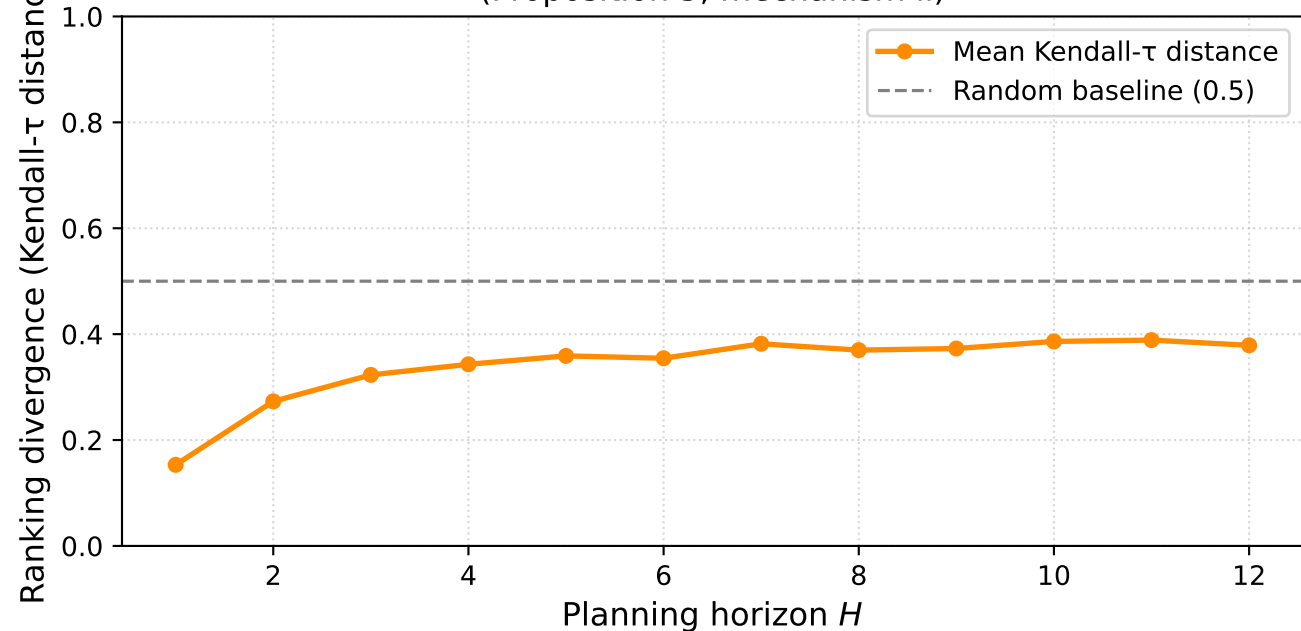
Action-Ranking Divergence: EHD vs Single-Step EFE (Proposition 5, mechanism ii)
