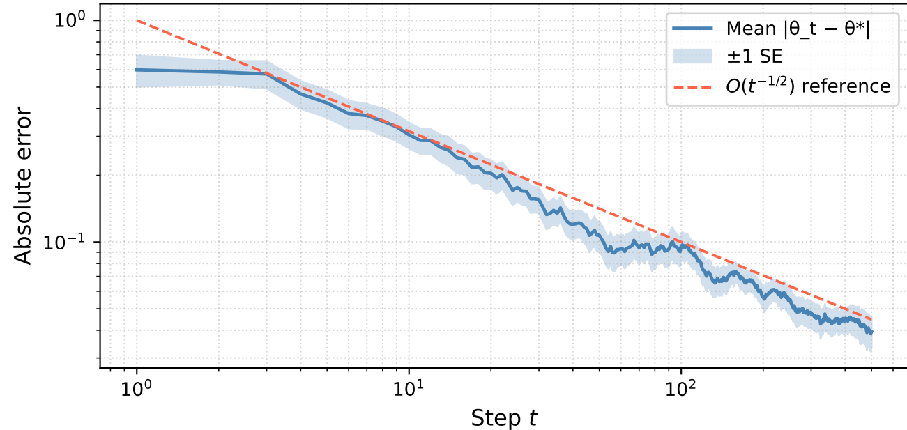
Robbins-Monro Convergence of EHD Recalibration Rule (Proposition 4)
