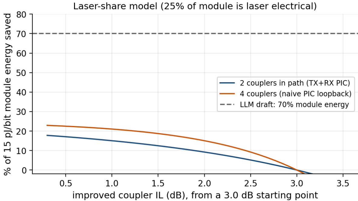
Figure 11. Module-energy fraction saved versus improved coupler IL. The 70% line is the archived claim.
