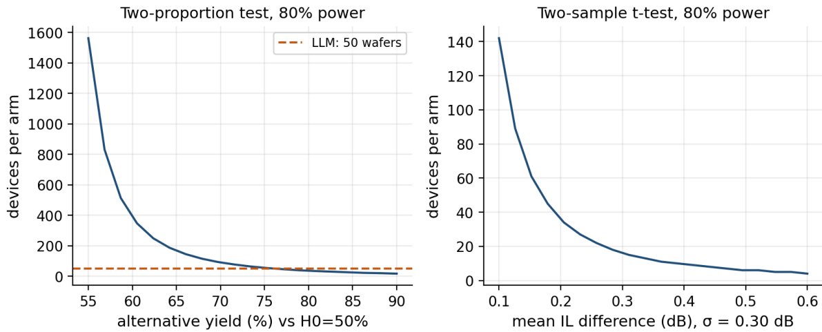
Figure 12. Device-level sample size. Fifty wafers is not the answer.
