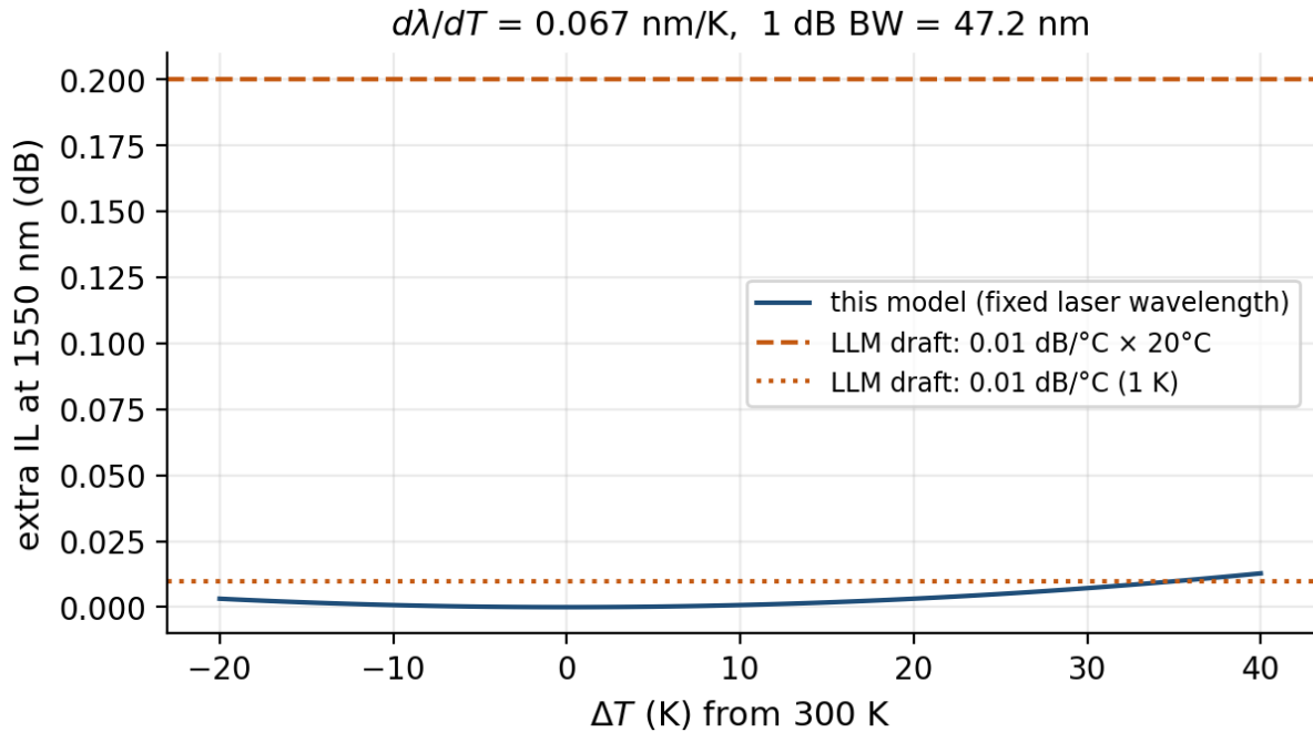
Figure 7. Extra IL at 1550 nm versus temperature. The archived 0.01 \text{ dB/}^\circ\text{C} \times 20^\circ\text{C} line is 0.20 dB.
