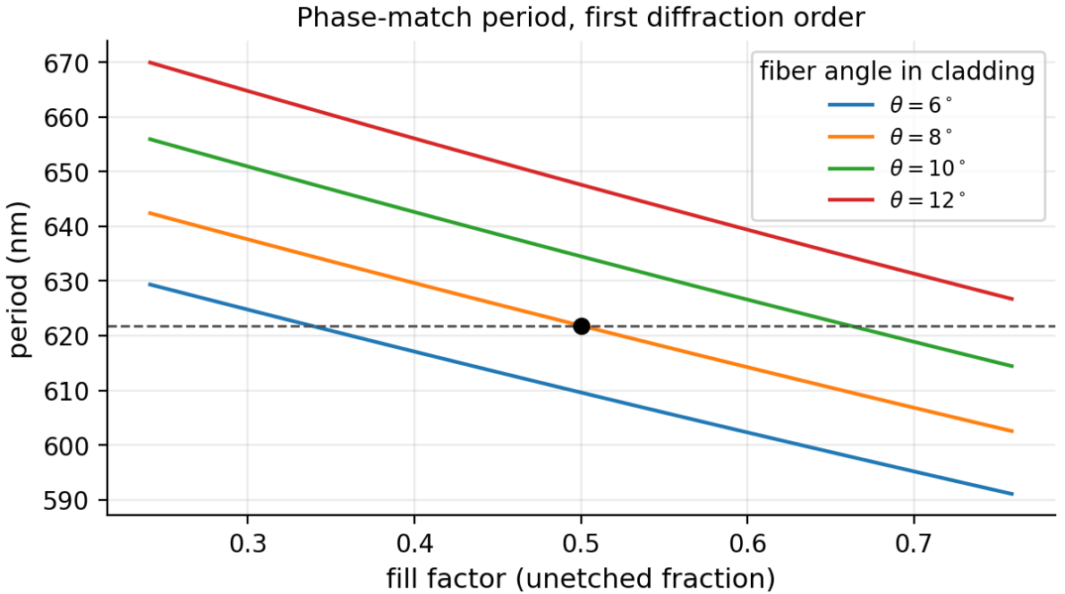
Figure 3. Phase-match period versus fill and fiber angle.
