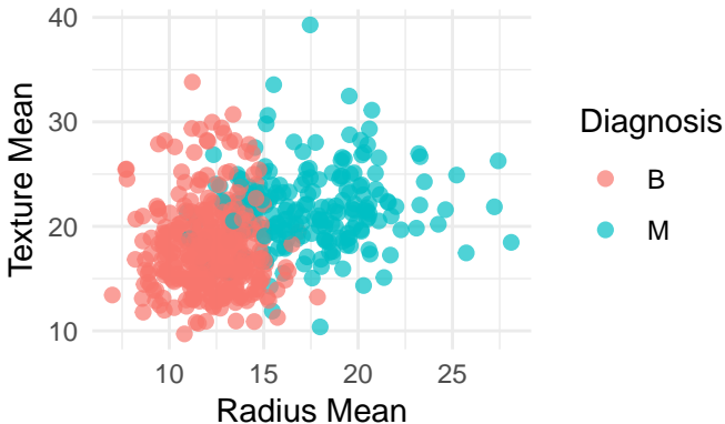
Scatter Plot of Radius Mean vs Texture
