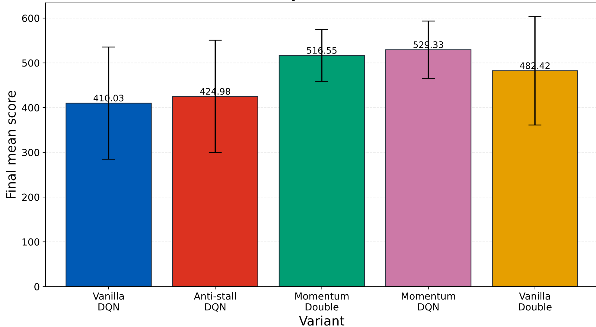
Final Score Comparison Across Variants
