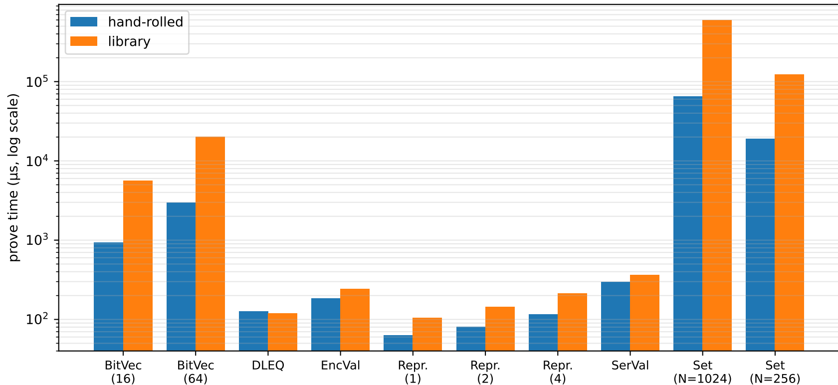
Hand-rolled vs library-backed — prove
