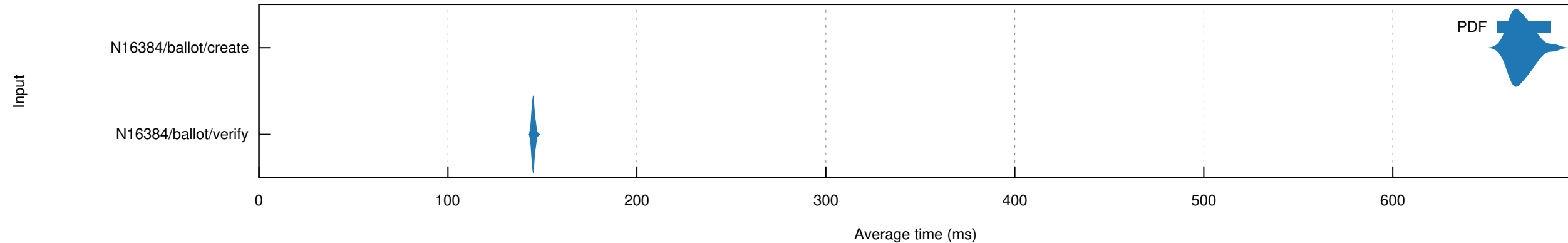
N16384/ballot: Violin plot
