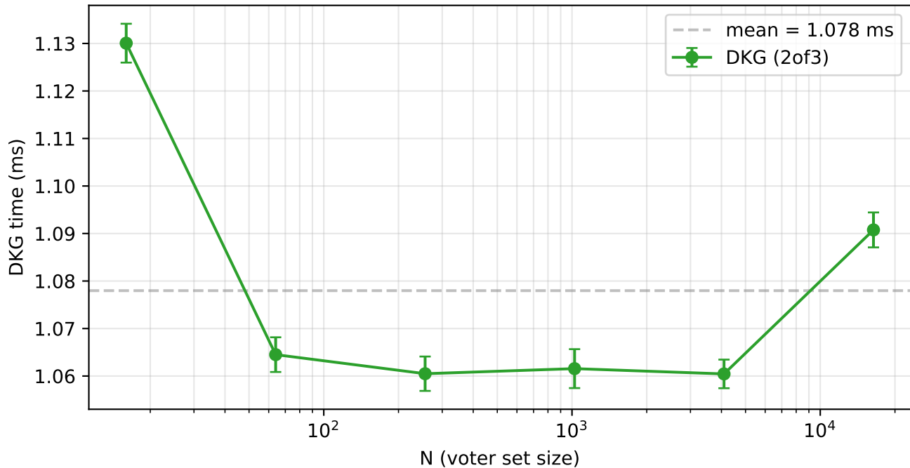
DKG cost is independent of N (3 authorities, threshold 2)
