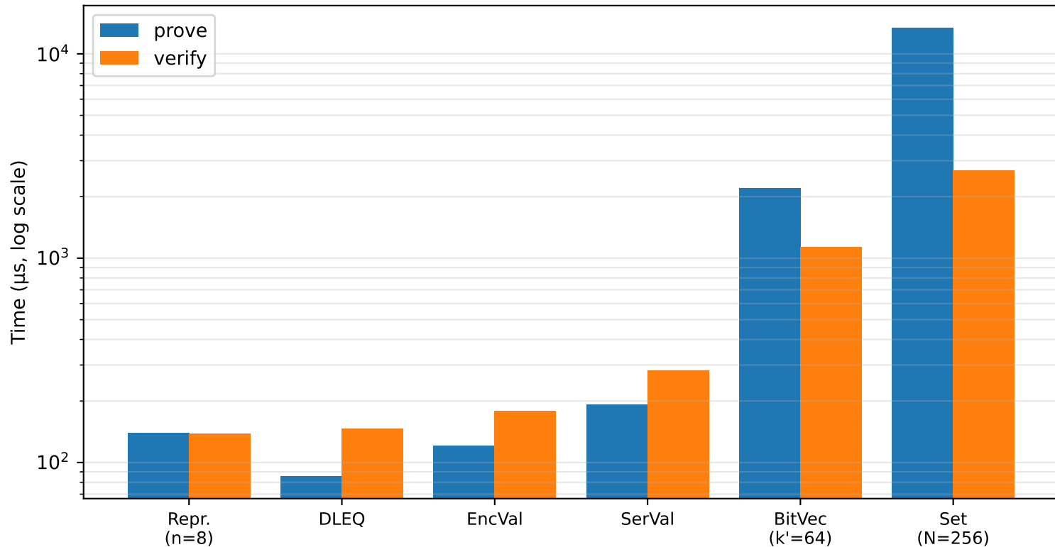
Per-proof prover/verifier cost (AWS, headline scale per proof)
