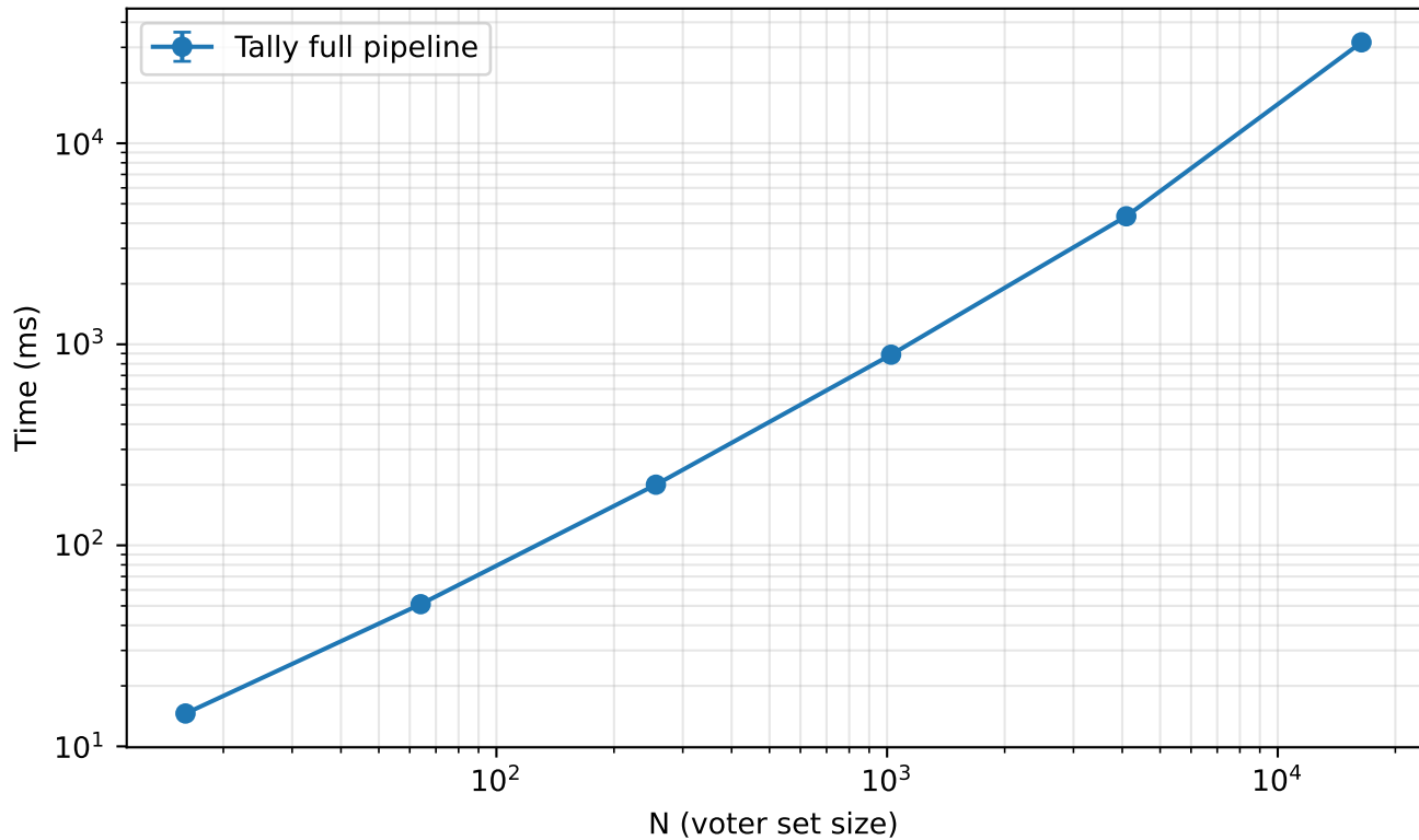
Tally full pipeline vs N
