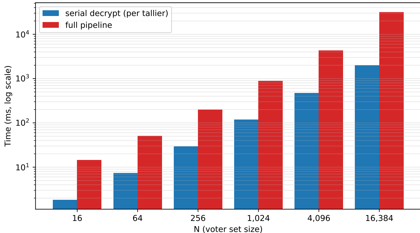
Tally pipeline: per-tallier serial decrypt vs full pipeline
