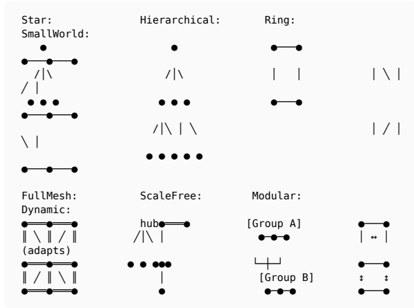
Listing 9: Visual representation of swarm topology patterns
