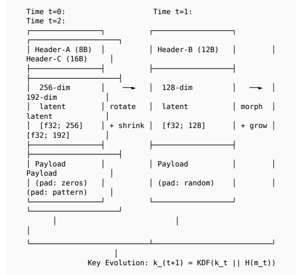
Listing 6: Chameleon Protocol: Moving-target message evolution
