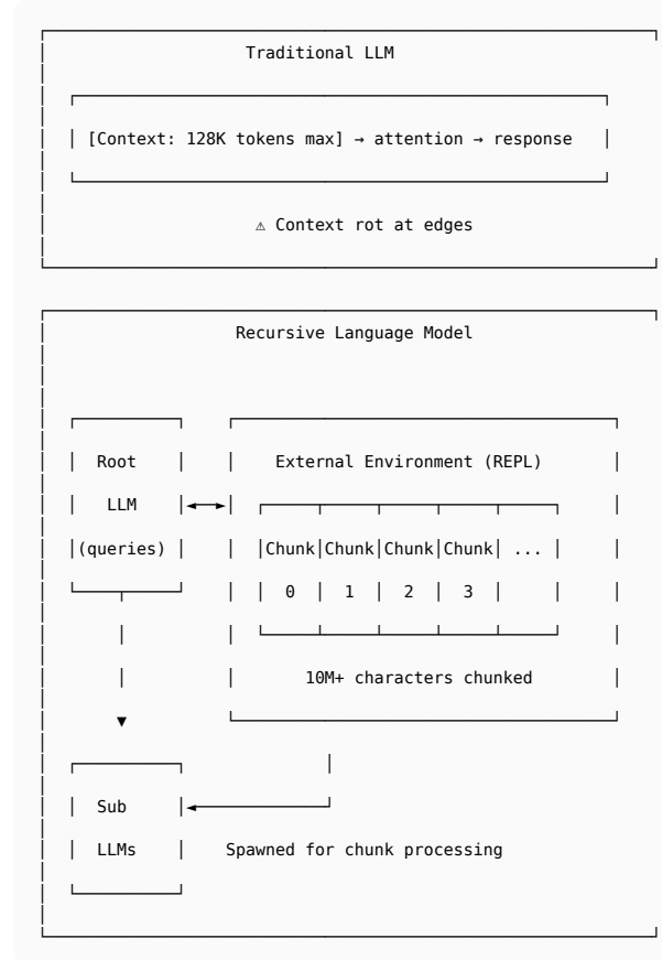
Listing 7: RLM architecture: context as external REPL environment
