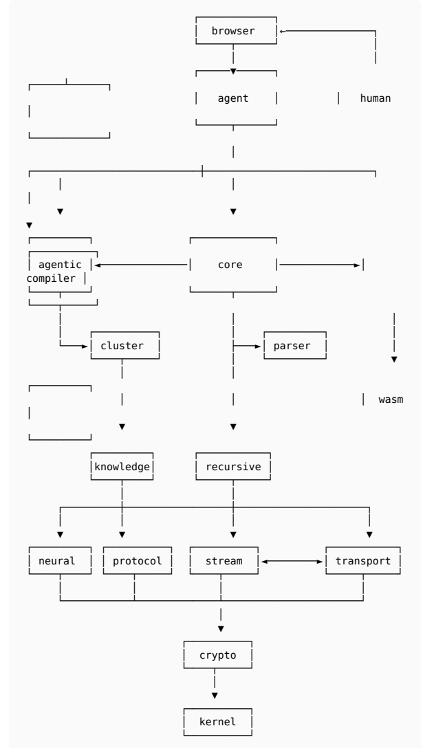
Listing 4: Crate dependency graph showing inter-crate relationships
