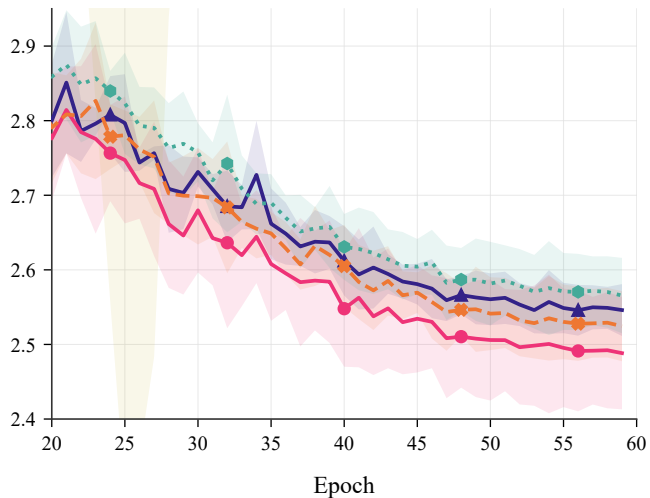
Convergence Detail (Epochs 20-60)
