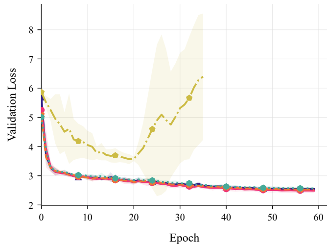
Full Training Dynamics
