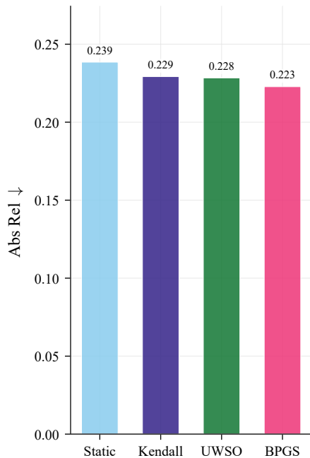
Depth
