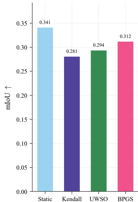
Segmentation
