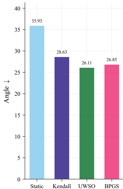
Surface Normals
