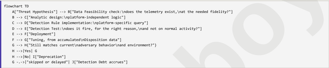
Figure 1.2 — The detection lifecycle, from hypothesis to deprecation. CONCEPTUAL. Illustrates the stage sequence this book assumes throughout; it is a process model, not a capture of any specific team's ticketing workflow. Part 37 (Detection Testing) expands the test stage; Part 42–43 (Detection Quality, Detection Debt) expand the tuning/deprecation loop and what accrues when it's skipped. Diagram ID FIG-01-02 .
