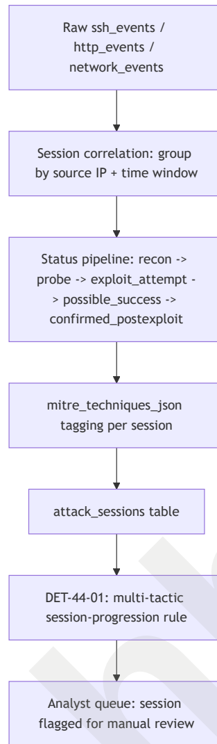
Figure 44.3 (FIG-44-03) — From raw event streams to a stage-progression alert. CONCEPTUAL. Illustrates the general data-flow shape behind DET-44-01 below — session correlation, then tactic tagging, then a rule evaluating the tagged session — as an architecture sketch of what the honeynet collector's real pipeline does, not a literal reproduction of its source code.
