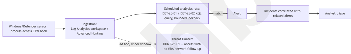
Figure 25.1 (FIG-25-01) — KQL detection and hunting data flow, Sentinel/Defender. CONCEPTUAL. Illustrates how the same underlying telemetry feeds both a bounded, scheduled KQL detection rule (DET-25-01 or DET-25-02) and a wider, ad hoc hunting query (HUNT-25-01) against the same tables, and where each path ends up (an incident queue versus a documented hunt finding). This is a data-flow sketch, not a capture from a real workspace. Rendered above; the Mermaid source above is the editable version of record.
