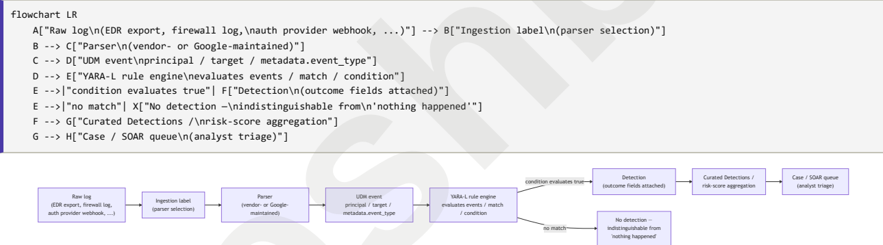
Figure 28.1 (FIG-28-01) — Data flow from a raw log to an analyst-facing detection in Google SecOps. CONCEPTUAL Illustrates the hop-by-hop path a YARA-L rule actually sits on: ingestion-label selection decides which parser runs, the parser decides what UDM shape the rule ever gets to see, and a rule that references a UDM field the parser never populates produces the same "no match" outcome as a rule with correct logic evaluated against activity that genuinely didn't happen. Not a capture from a live tenant; it is a structural diagram of the pipeline described in this section and in Part 6 generally.
