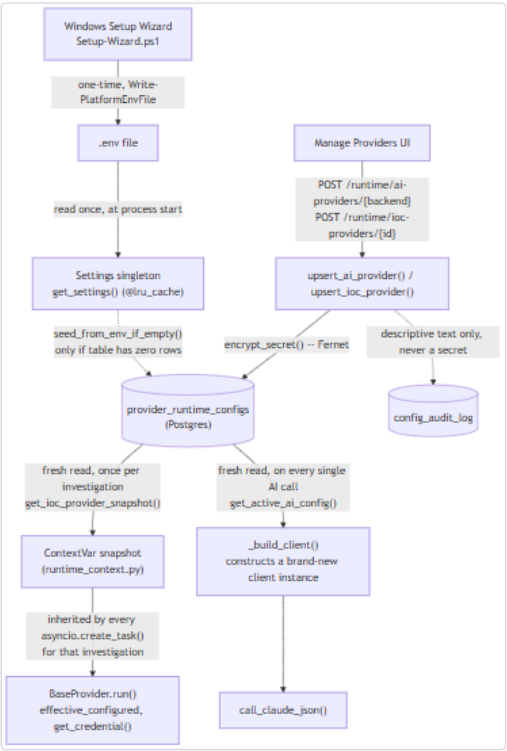
Figure 5 — Diagram: Audit trail Diagram: Credential lifecycle -- wizard/ .env and runtime-API entry points, encrypted storage, the per-investigation ContextVar snapshot for IOC providers, and the per-call fresh client construction for AI backends. The two right-hand branches are why a saved credential change needs no restart: neither path ever reads a value cached longer than one investigation (providers) or one call (AI backends).
