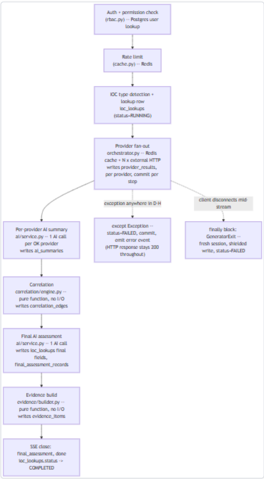
Figure 3 — Diagram: Summary of the full path Diagram: POST /api/v1/lookup/stream , end-to-end sequence. Each stage after provider fan-out commits its own writes independently, so a mid-stream failure or disconnect only loses the one step in flight, never everything already completed. Every other endpoint in the platform ( analysis.py 's why/what-is/disagreement/etc., hunting.py , pivot.py , basket.py , cases.py ) operates on an already-completed lookup's persisted rows and follows the same routes → domain-module → models layering, but without the streaming/session-ownership complexity described above, since none of them return a StreamingResponse — they load, call one domain function, and return a single JSON body.
