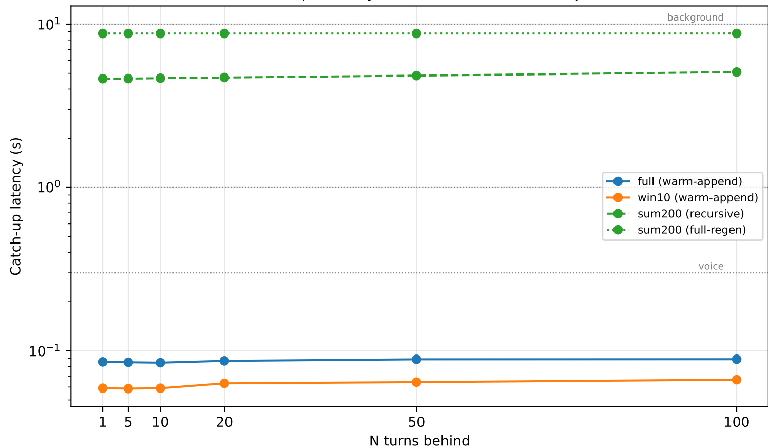
E32: Catch-up Latency vs Staleness — LoCoMo (qwen7b)
