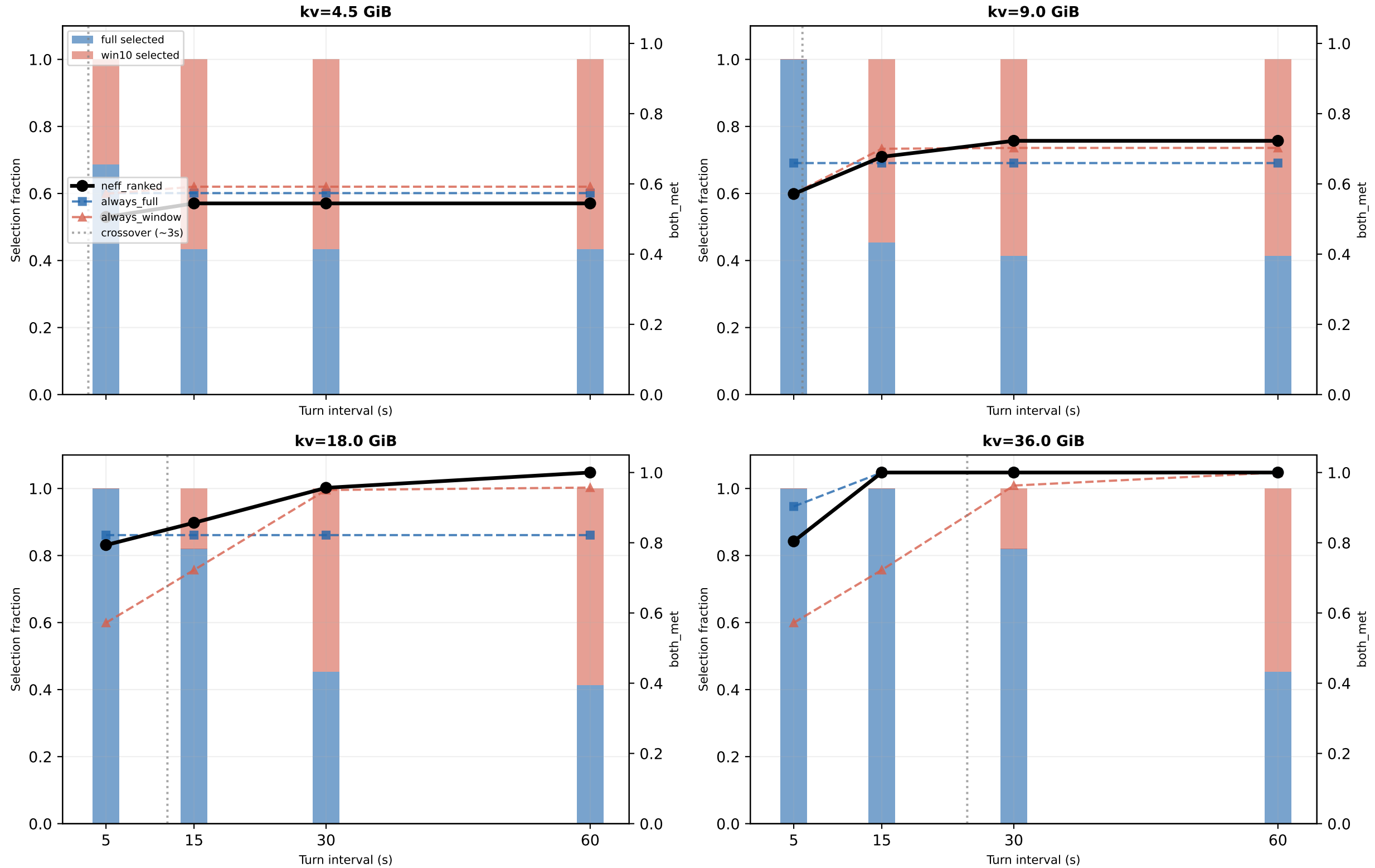
E36f: neff_ranked selection vs turn interval (bars = fraction selecting full/win10; lines = both_met outcome) locomo, q=0.20, ttft=1000ms, n=50
