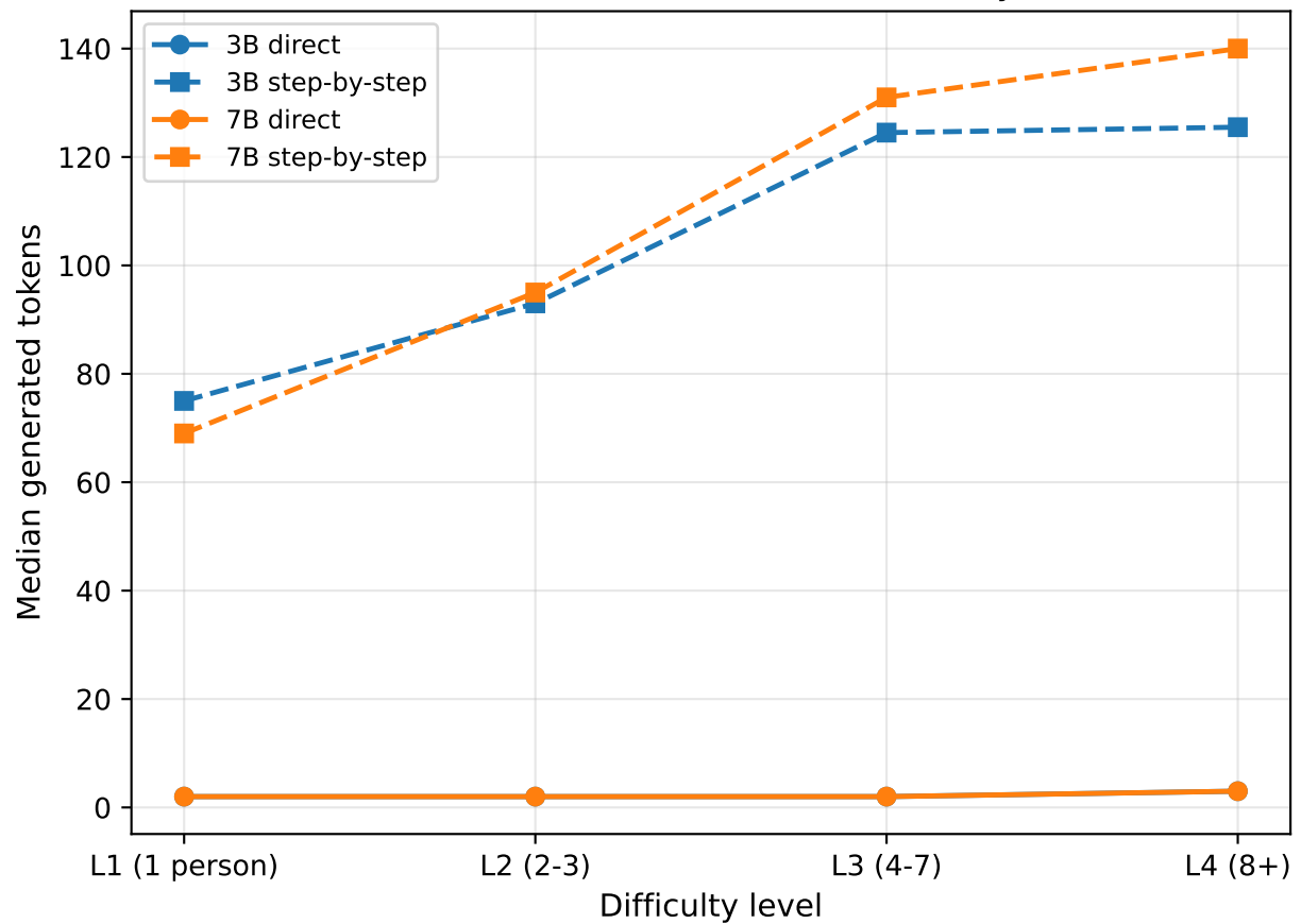
Generated Token Count vs Difficulty
