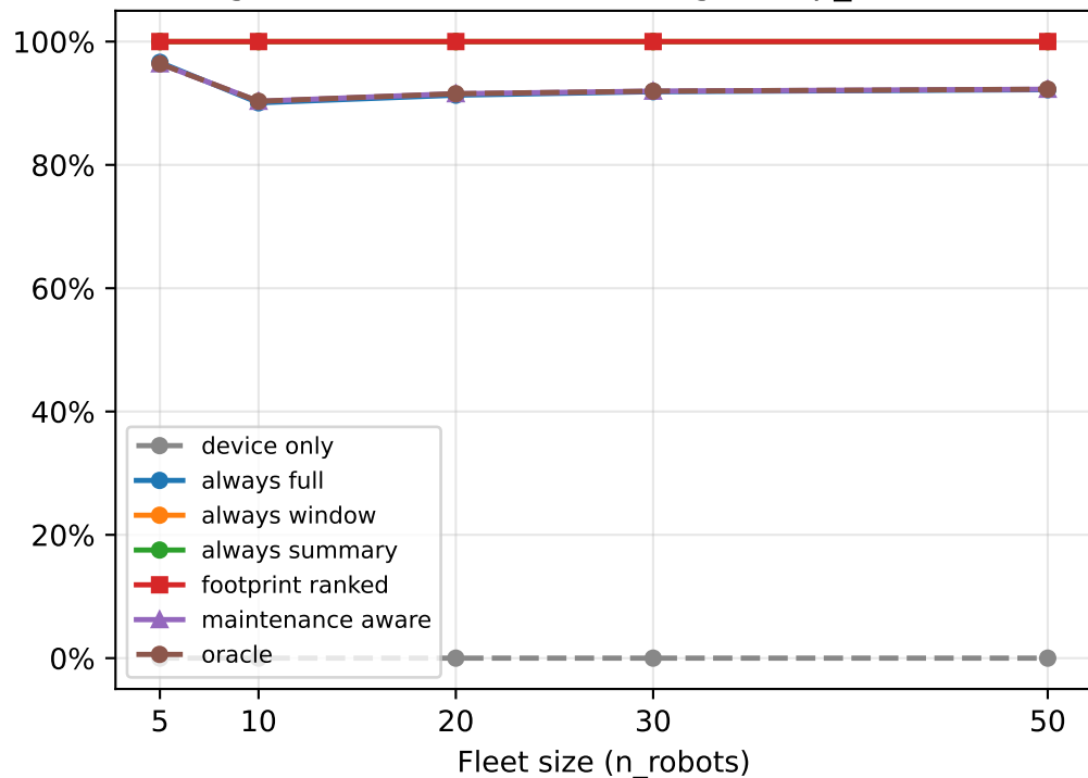
Egoschema — 1000 ms budget, cap_frac=0.5
