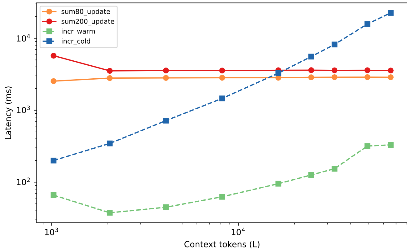
Update latency vs context length
