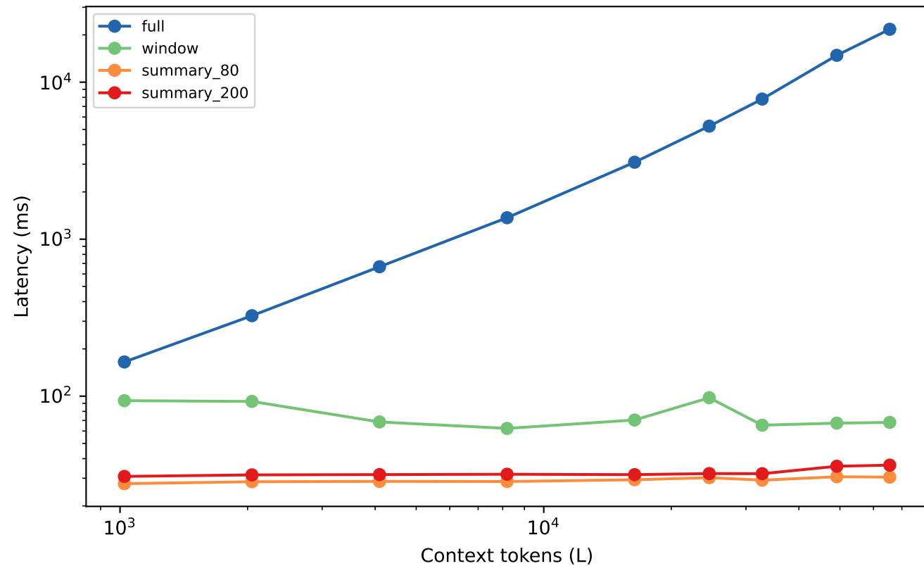
Restore latency vs context length
