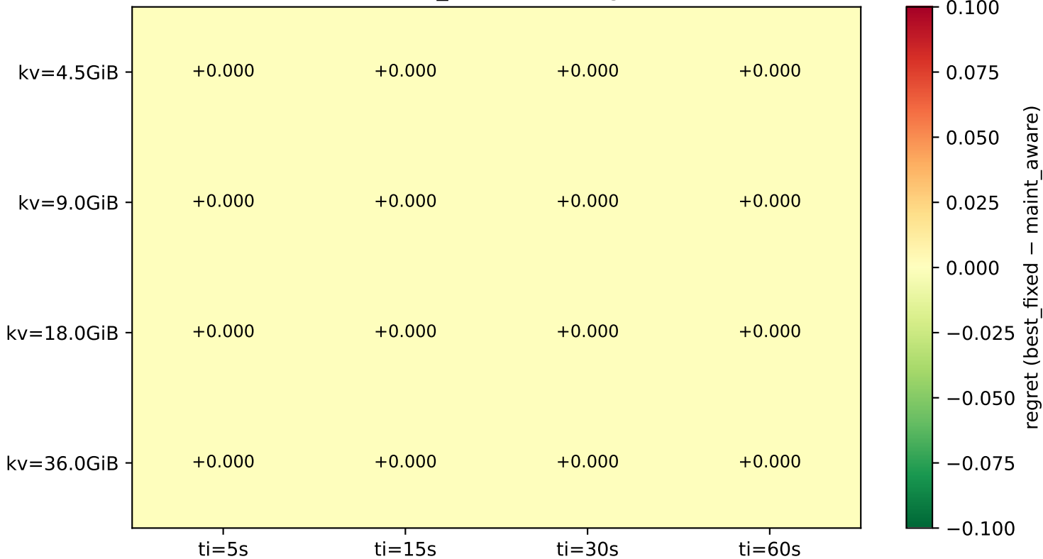
S2 Regret: best_fixed – maintenance_aware LoCoMo q=0.20, ttft=1000ms, n=50 (red=maintenance_aware worse; green=better)
