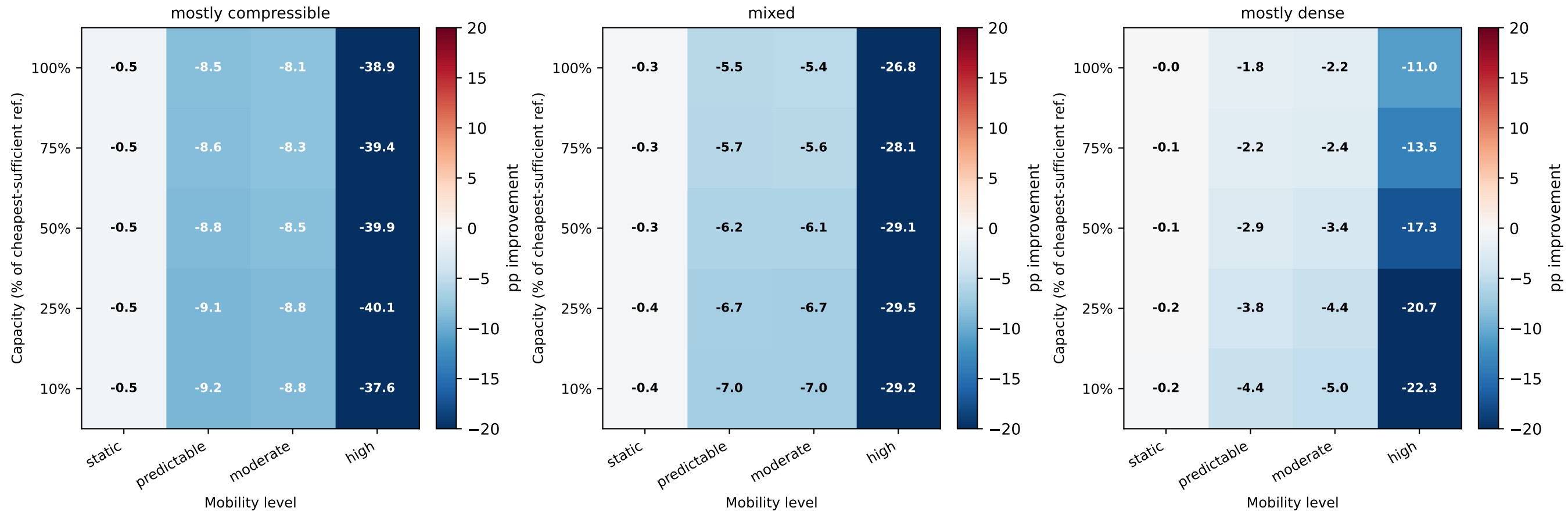
E24b: joint improvement over fidelity_only (pp) (averaged over \tau \in \{0.80, 0.90, 0.95\} \times \text{drift} \in \{0, 20\} )
