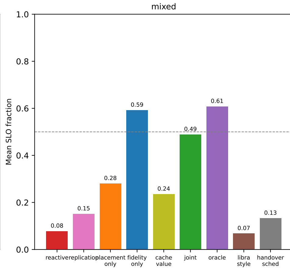
E24b: Mean SLO fraction by policy (averaged over cap × mobility × tau × drift)
