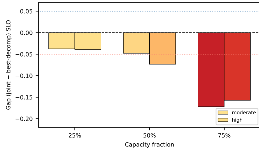
tau=0.95, mixed
