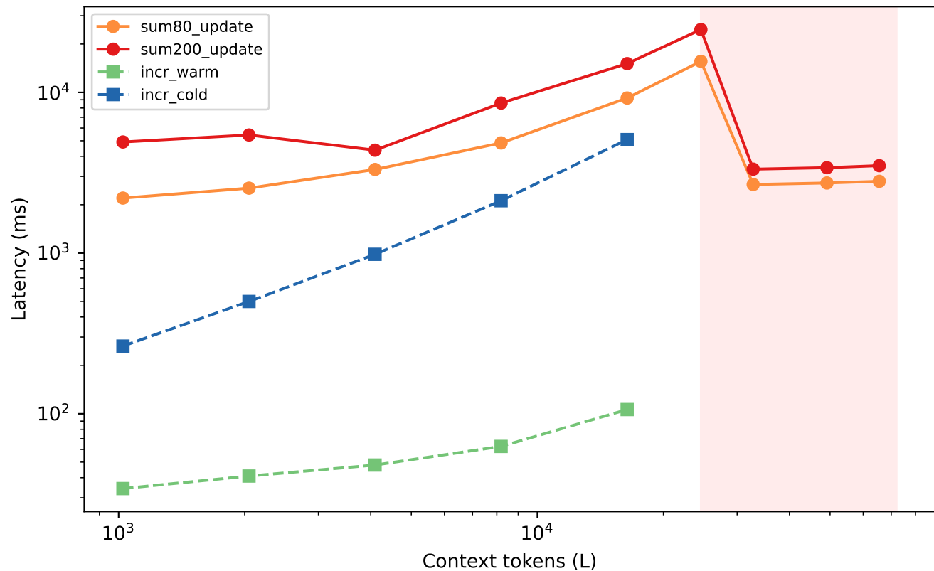
Update latency vs context length (full-context input)
