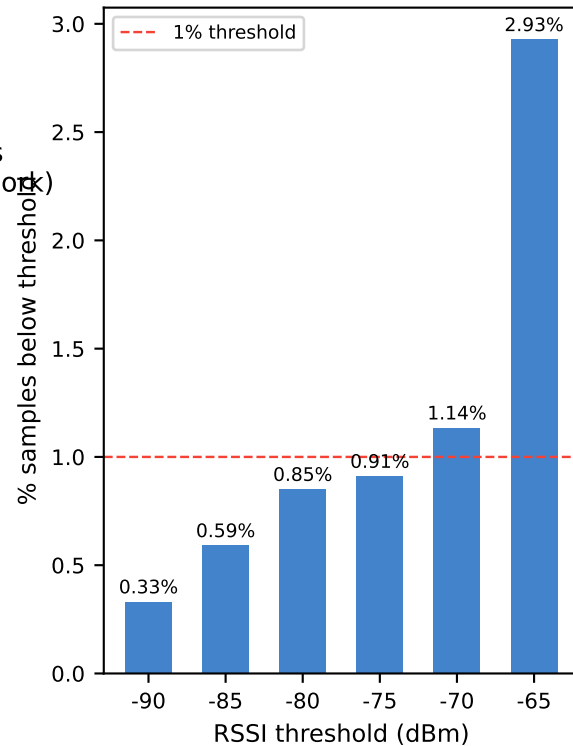
(C) Indoor robot WiFi (herolab, n=16,540)
