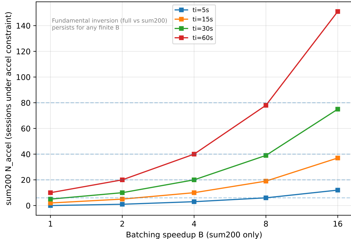
Batching sensitivity for sum200 (dashed = win10 reference at each ti)
