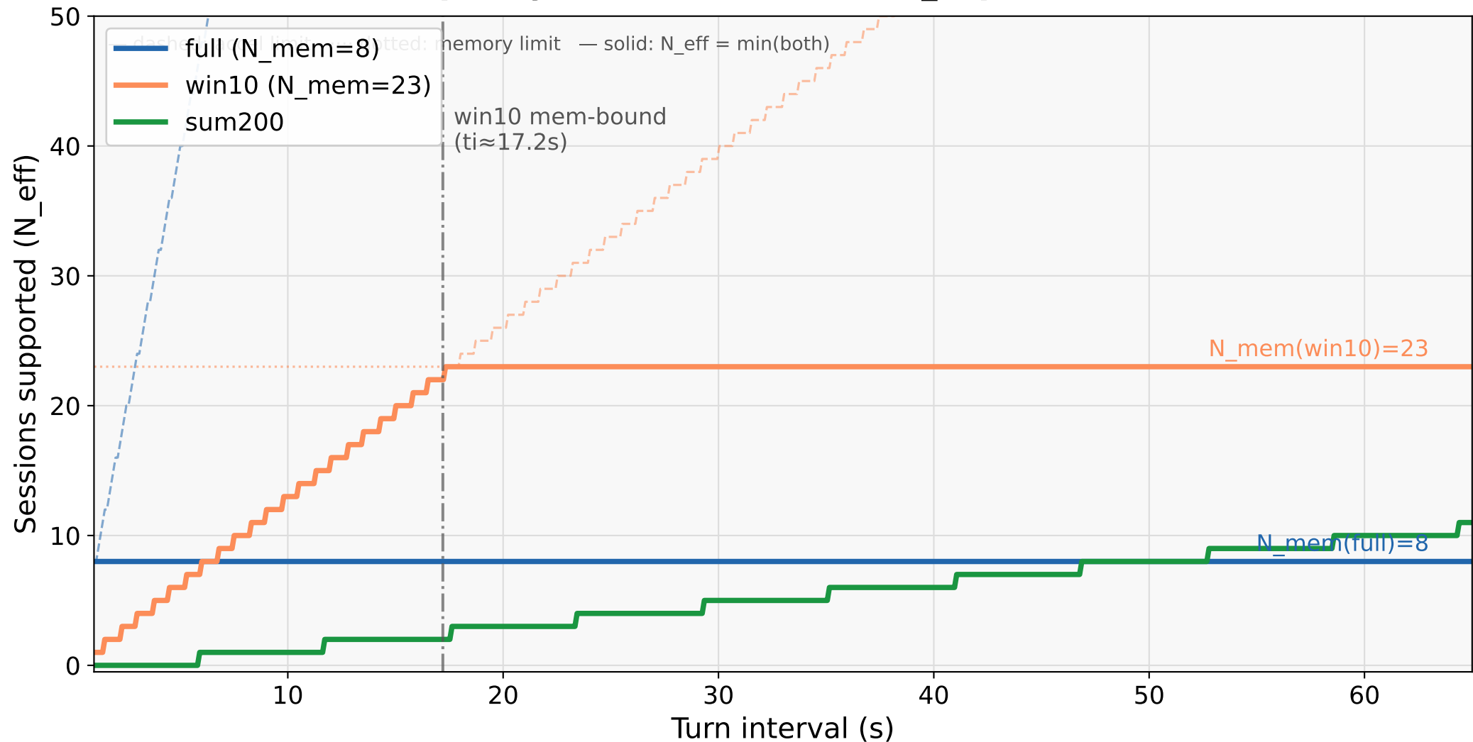
Effective capacity vs turn interval (kv_cap=9.0 GiB, LoCoMo)
