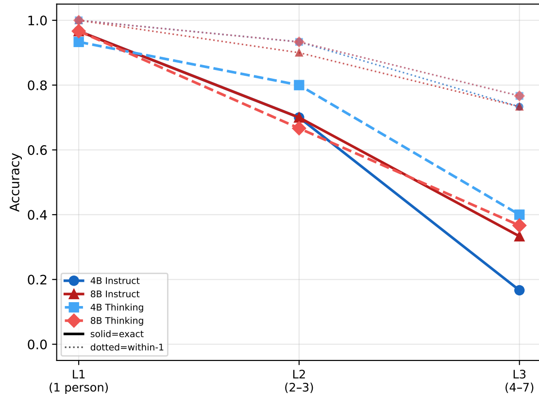
Accuracy vs Difficulty (L1-L3)
