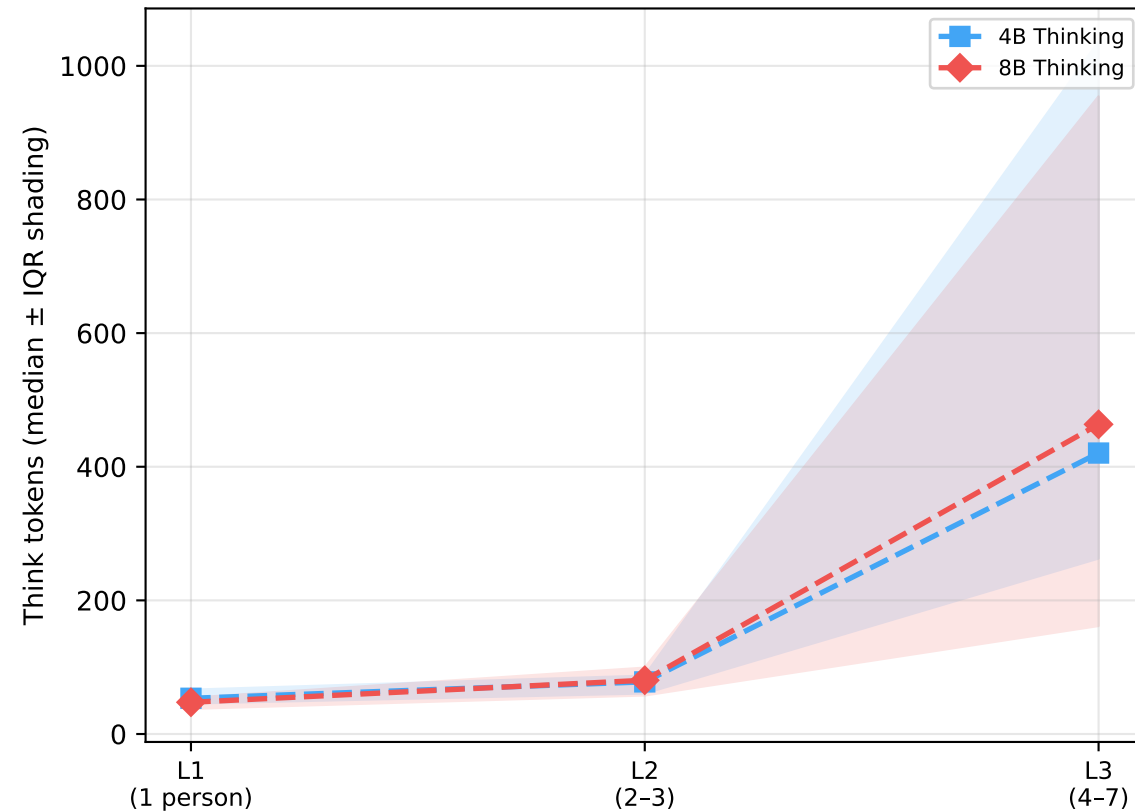
Reasoning Length vs Difficulty
