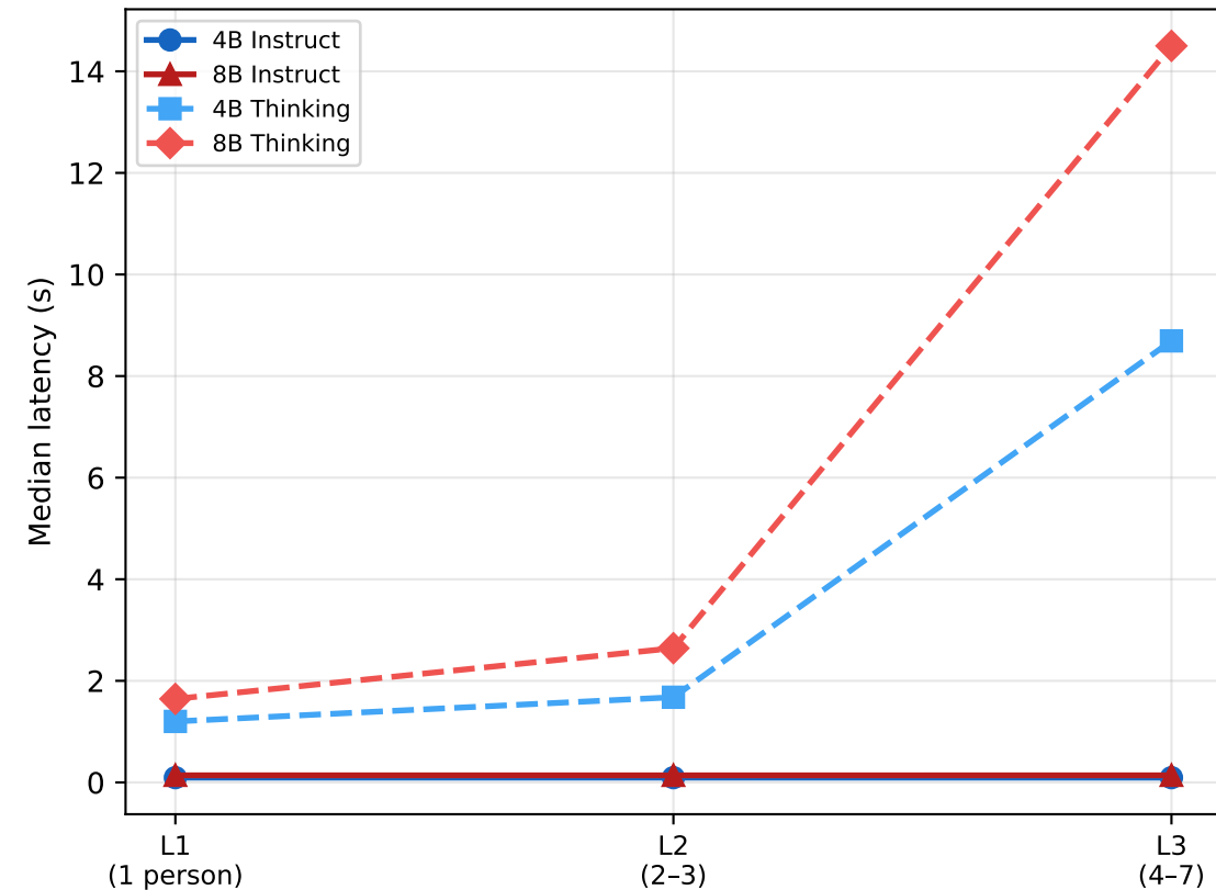
Latency vs Difficulty
