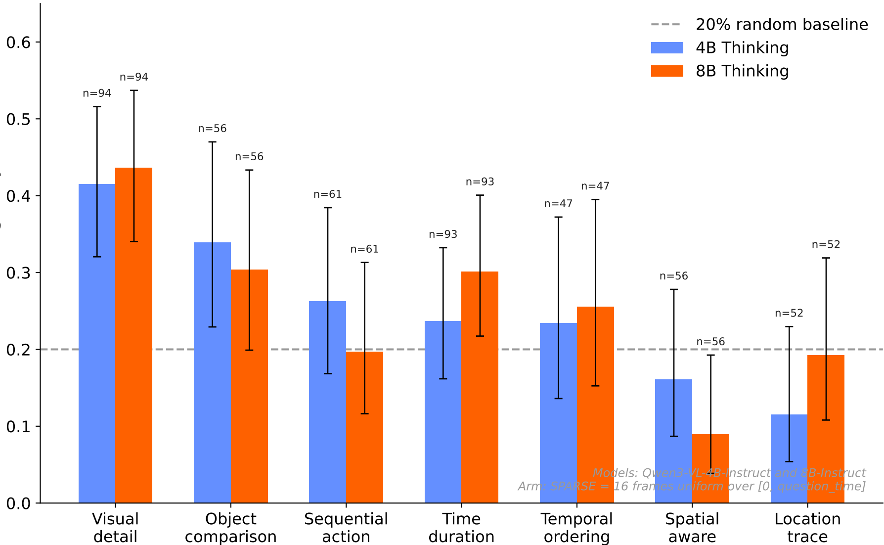
Accuracy — SPARSE arm (16 frames uniform, greedy decode)
