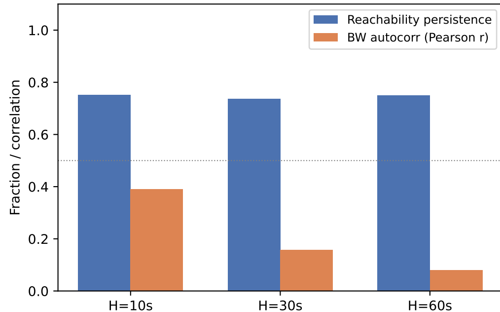
Predictability at horizons H=\{10,30,60\} s (Irish 5G, 16 Driving sessions)
