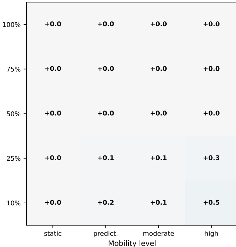
Joint SLO improvement (vs best non-joint baseline)
