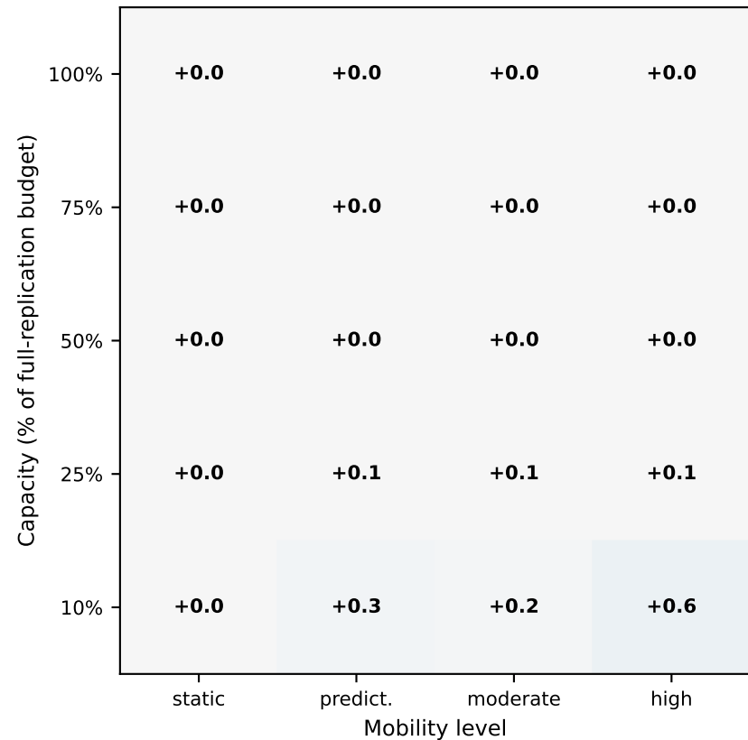
Mostly Compressible
