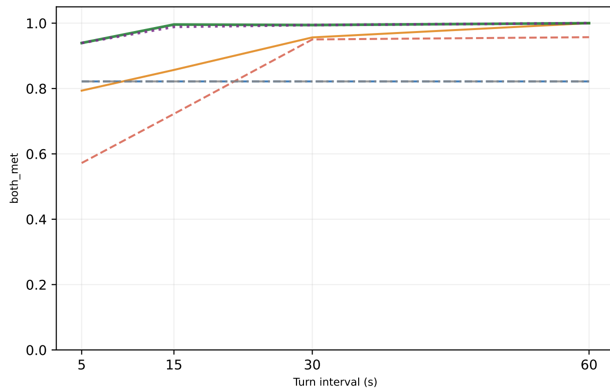
kv=18.0 GiB
