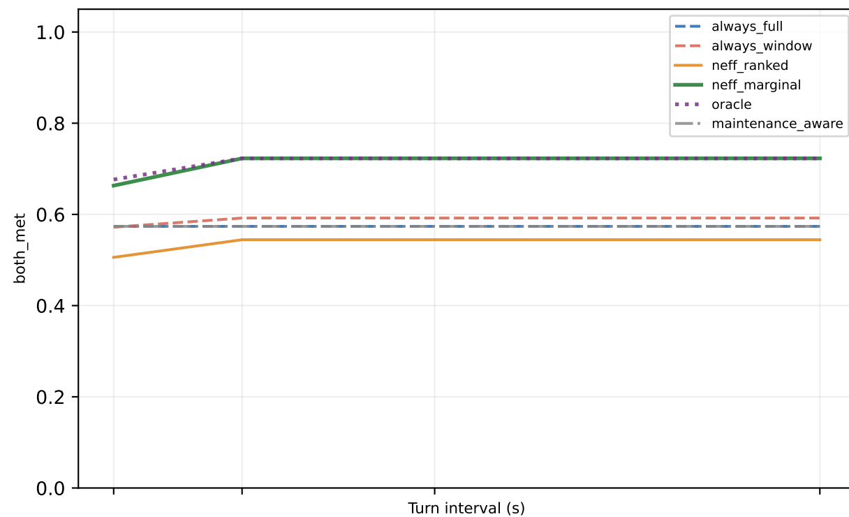
kv=18.0 GiB
