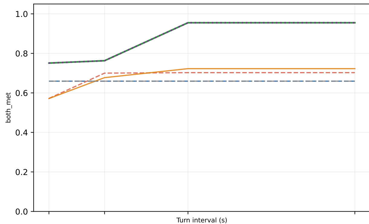
kv=36.0 GiB
