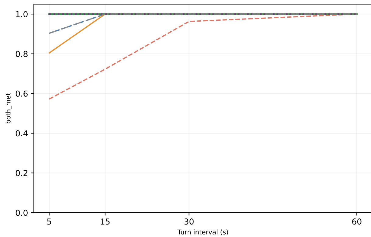
kv=36.0 GiB
