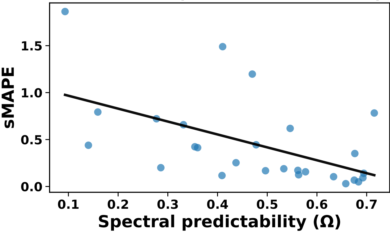
sMAPE vs. \Omega (dataset-level means)
