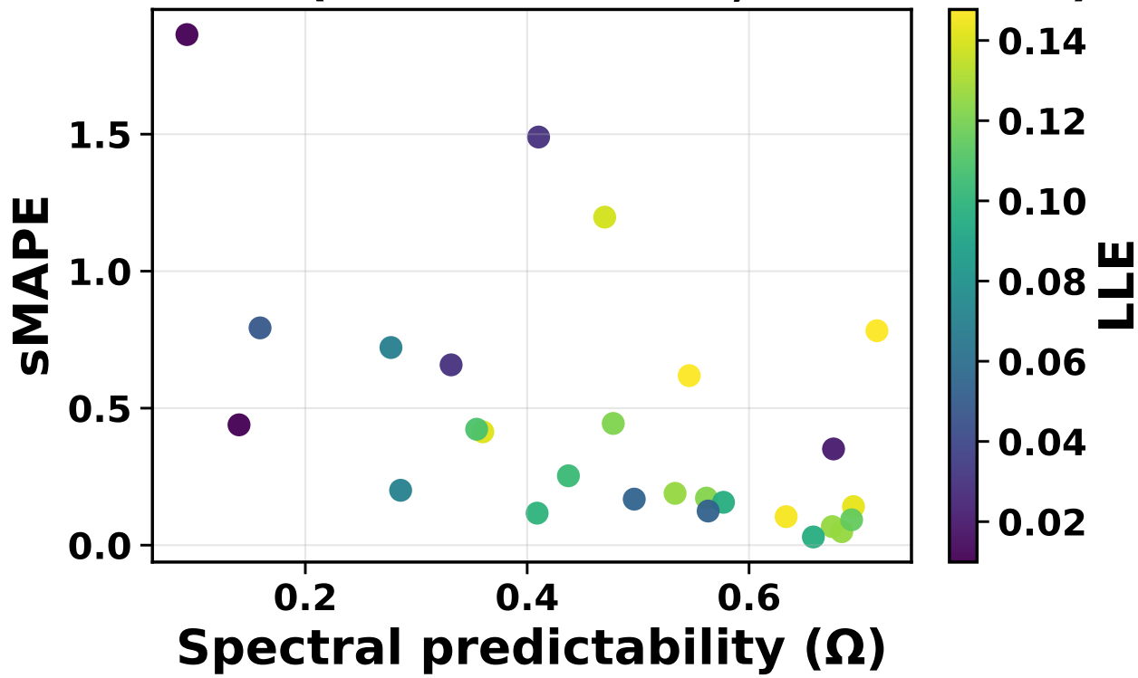
sMAPE vs \Omega (dataset means, color = LLE)
