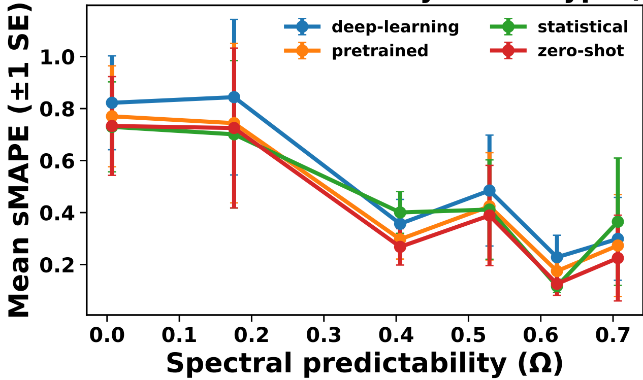
Binned trend of sMAPE vs \Omega by model type (filtered)
