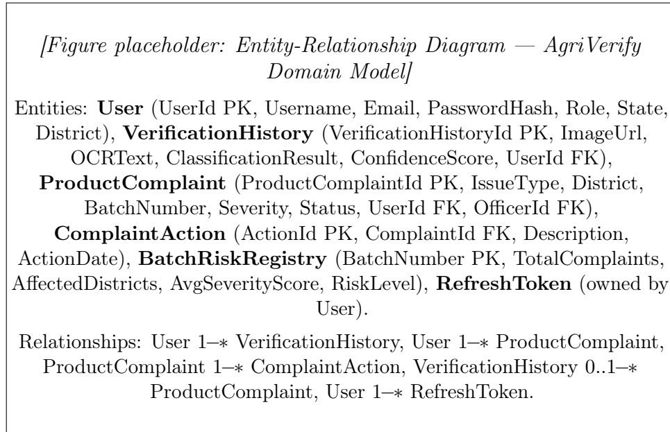
Figure 3.3: Simplified entity-relationship diagram for the AgriVerify domain model. Cardinality notation follows UML conventions.
