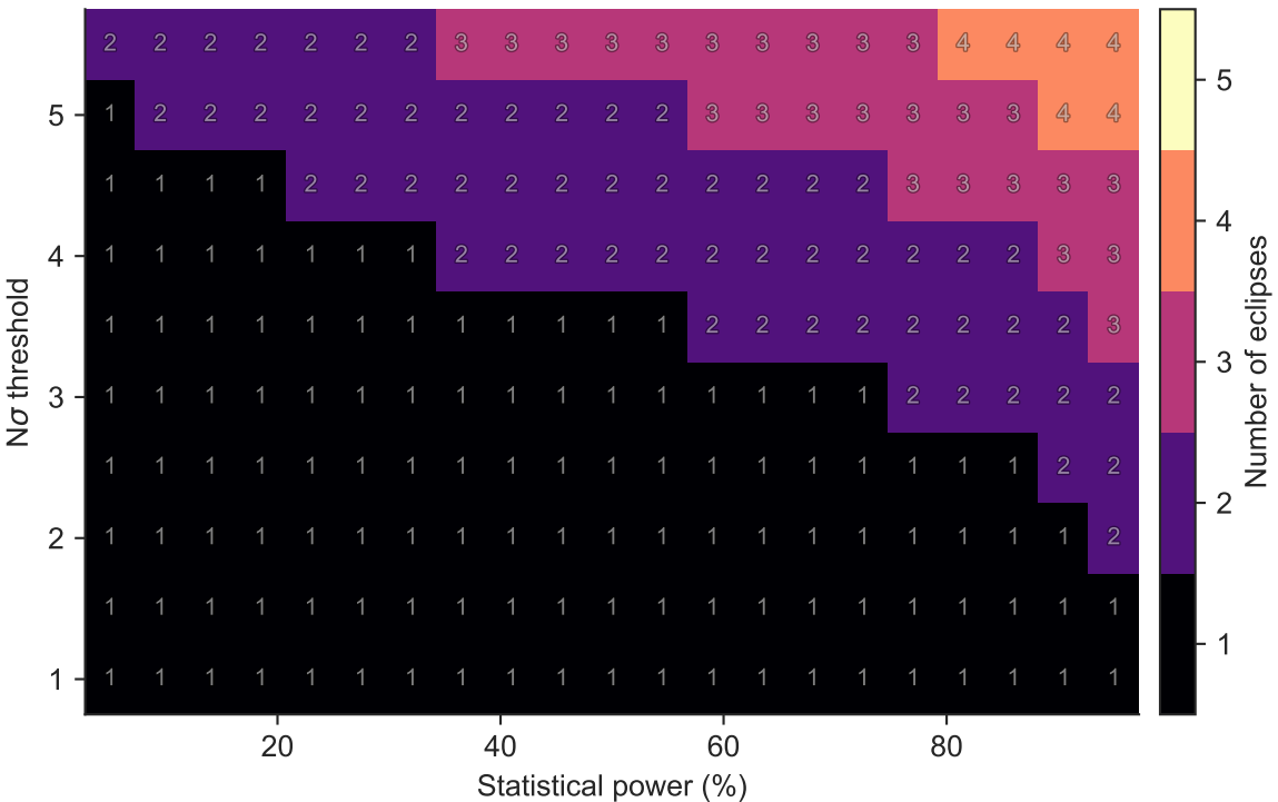
Checkpoint 2 Eclipses for LTT 1445 A c
