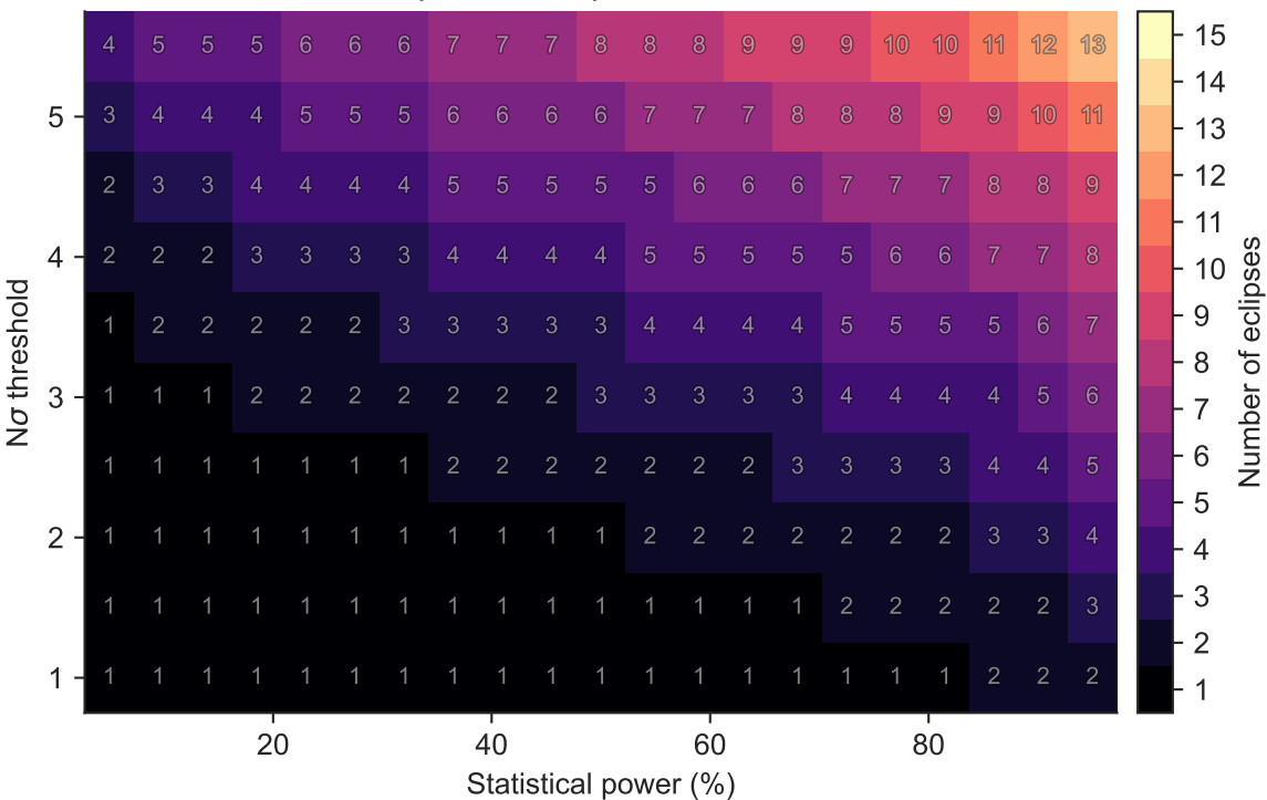
Checkpoint 2 Eclipses for TOI-771 b
