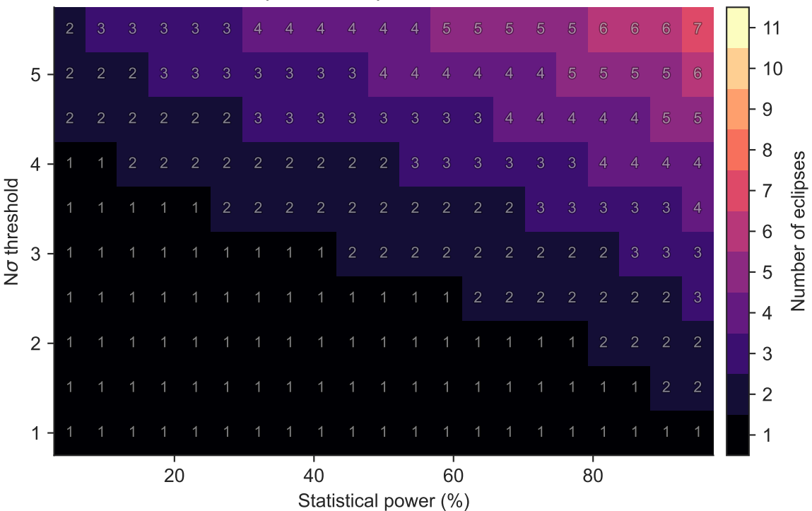
Checkpoint 1 Eclipses for GJ 3929 b
