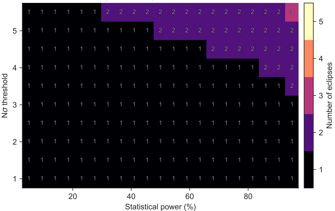
Checkpoint 2 Eclipses for LTT 1445 A b
