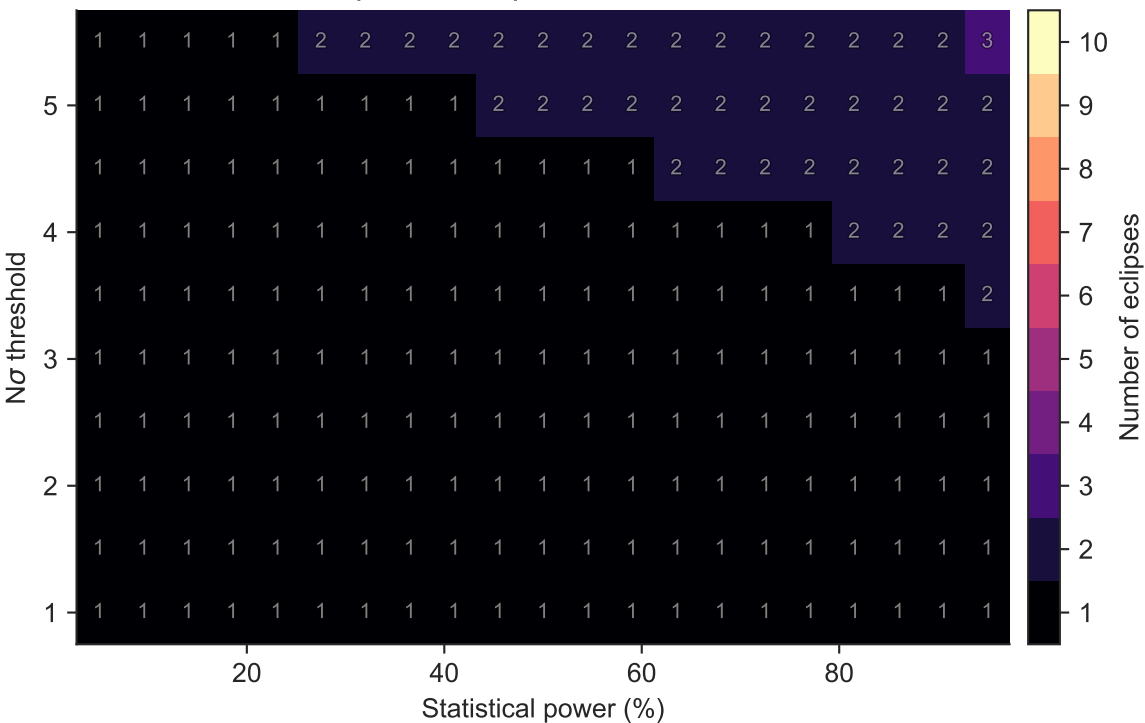
Checkpoint 1 Eclipses for HD 260655 c
