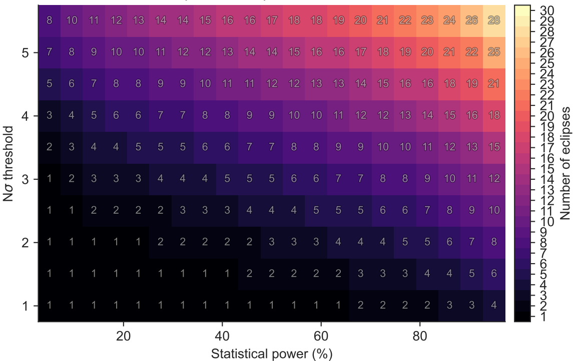
Checkpoint 1 Eclipses for TOI-1452 b
