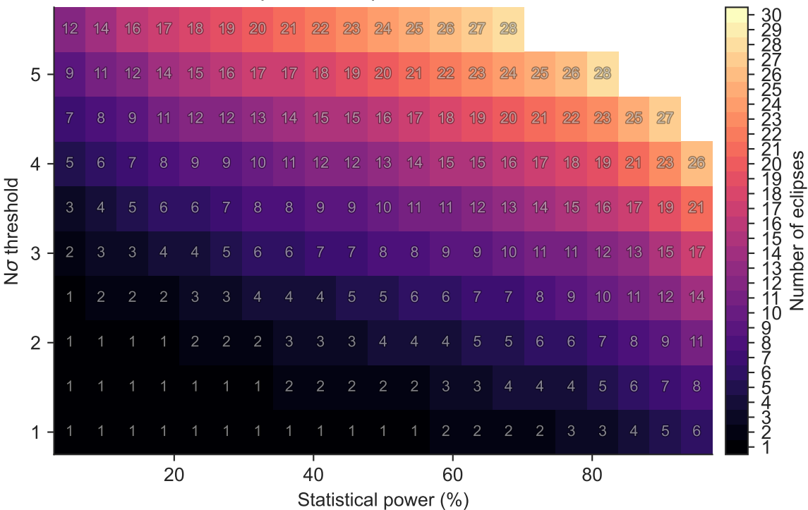
Checkpoint 2 Eclipses for TOI-1452 b
